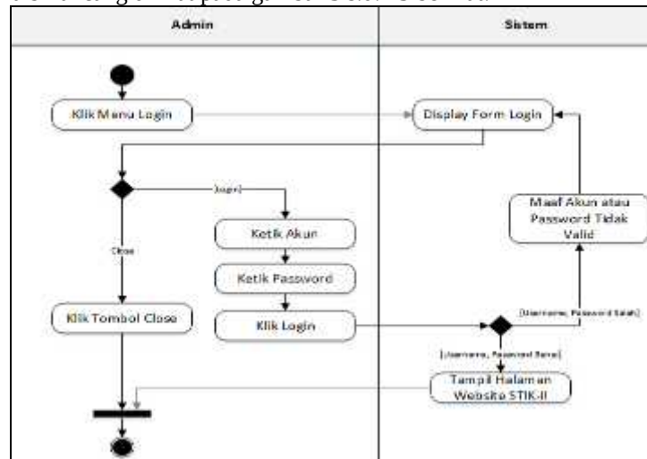
Gambar 3. Rancangan activity diagram proses login
