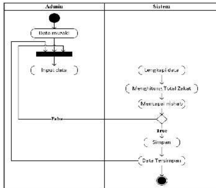
Gambar 3.7 Rancangan Activity Diagram Penerimaan Zakat Mal
