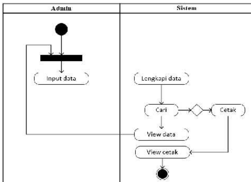
Gambar 3.8 Rancangan Activity Diagram Laporan Zakat
