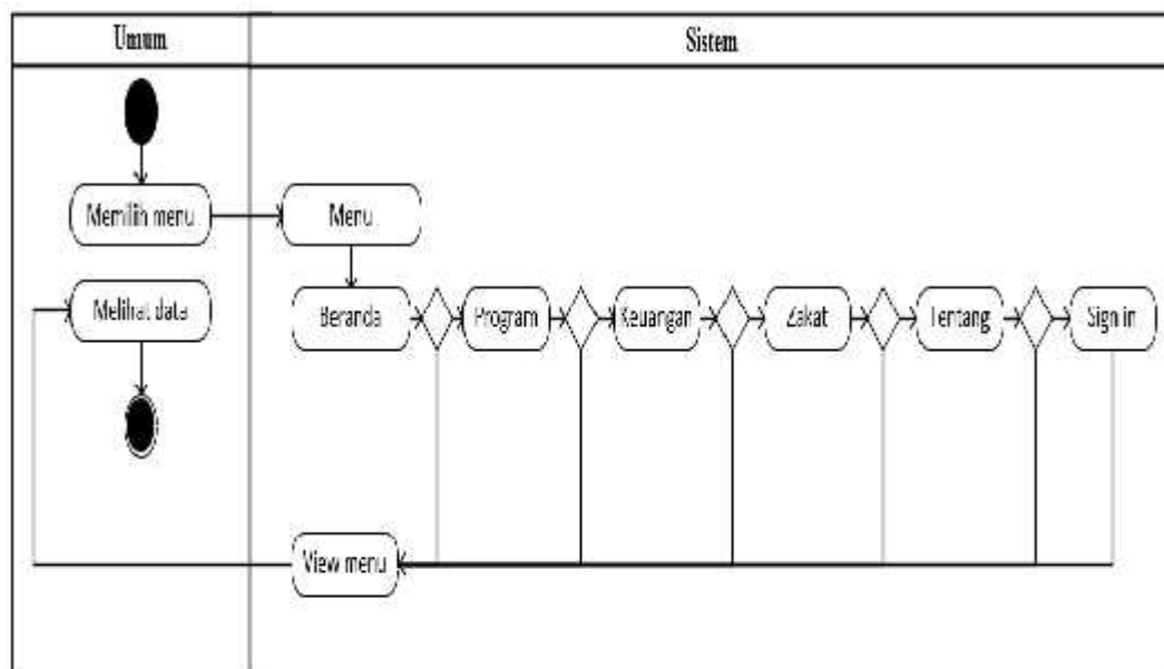
Gambar 3.3 Rancangan Activity Diagram User Umum Admin
