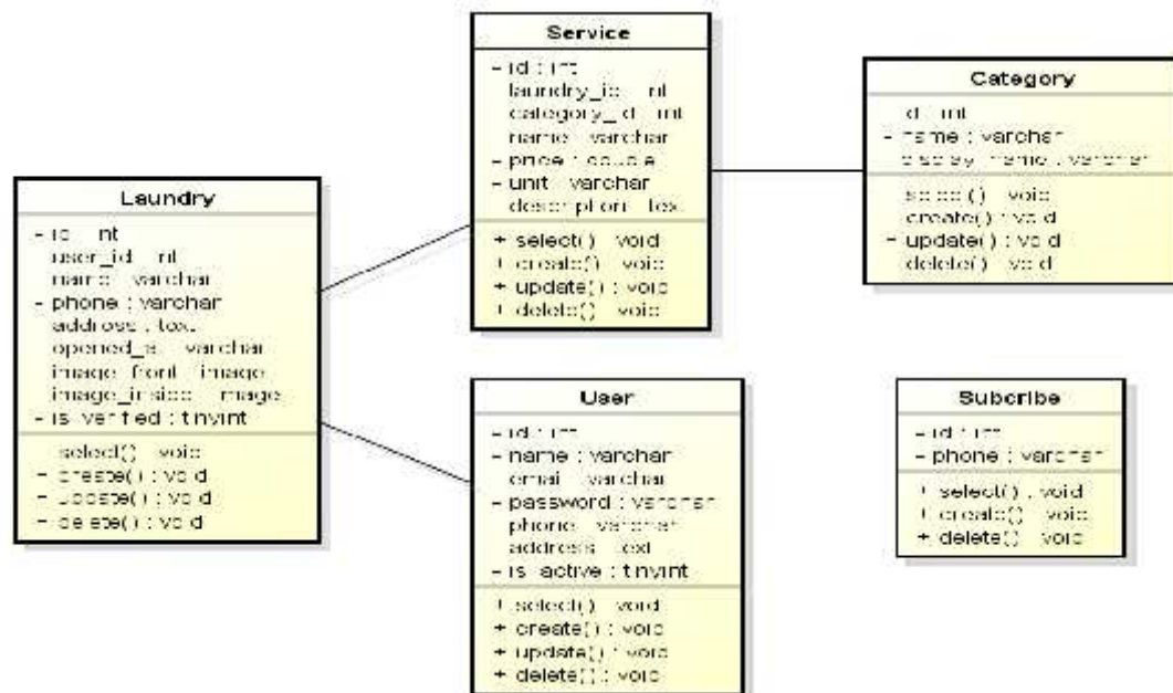
Gambar 4 Class Diagram Progressive Web Apps Pencarian Tempat Laundry
