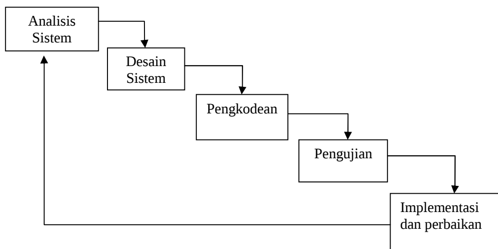
Gambar 1 Metode waterfall
