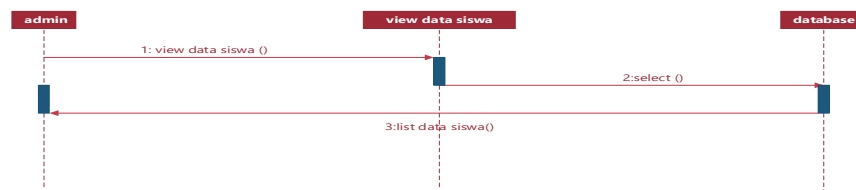
Gambar 1.8 Sequence Diagram Menu Siswa Admin
