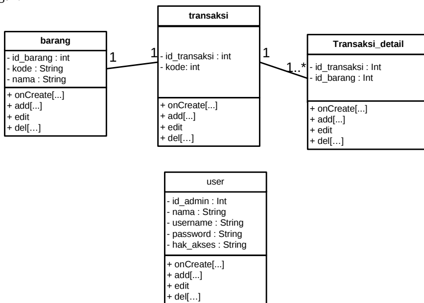
Gambar 2. Class Diagram Sistem
