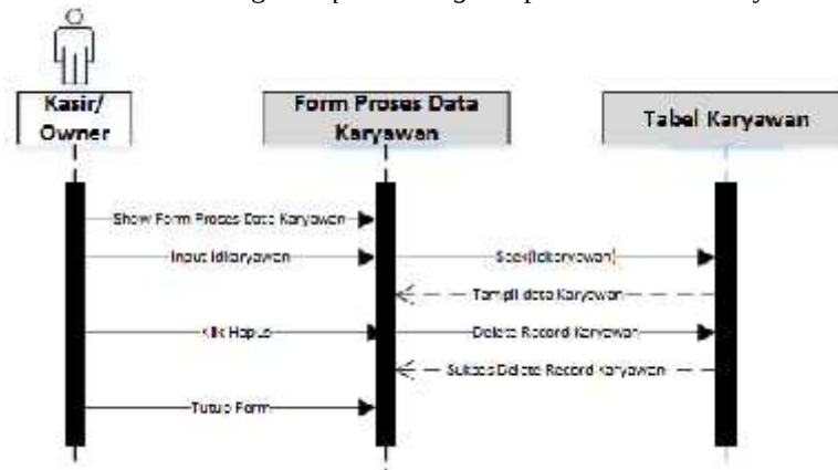
Gambar 7. Rancangan sequence diagram proses hapus data karyawan
