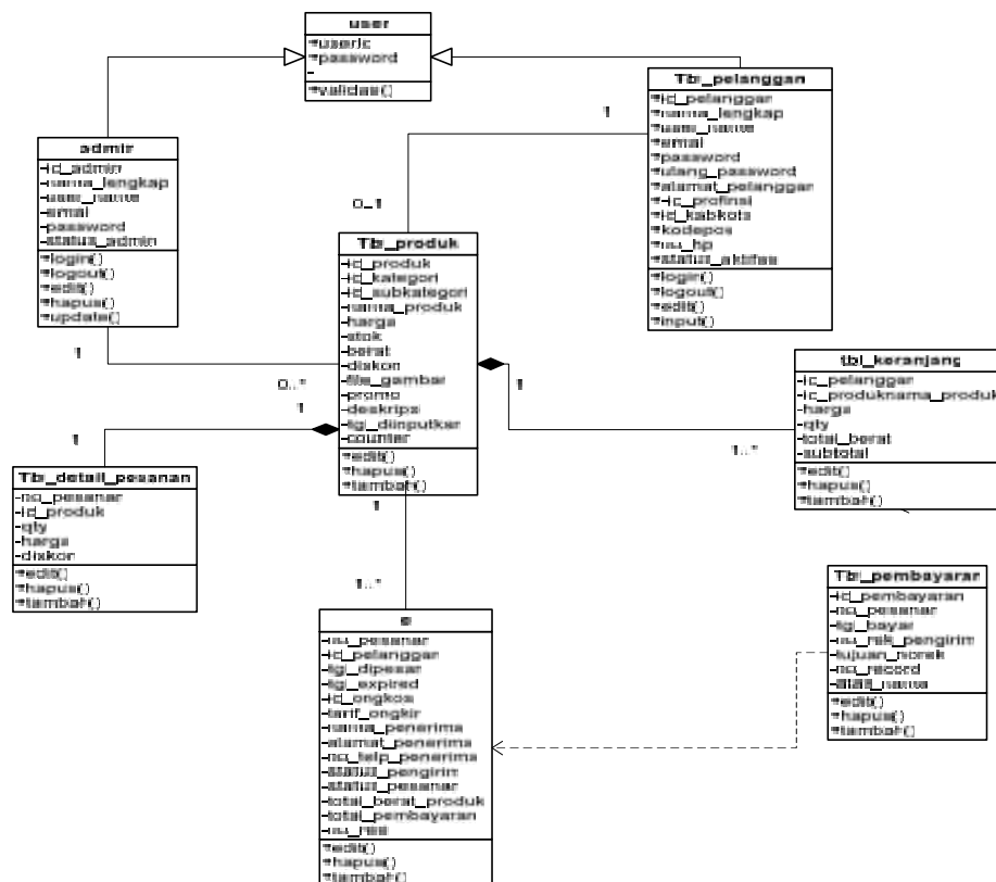
Gambar 4. Class Diagram
