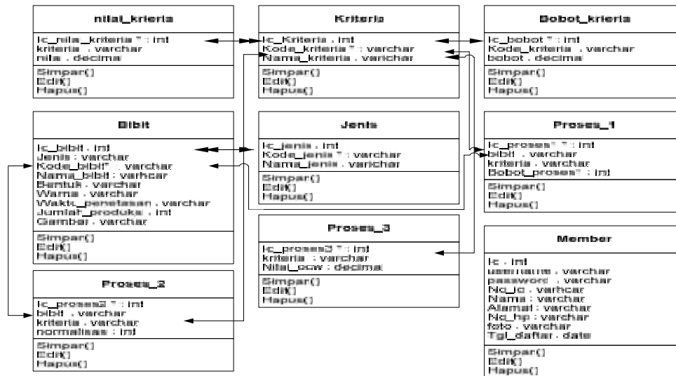
Gambar 2 Class Diagram
