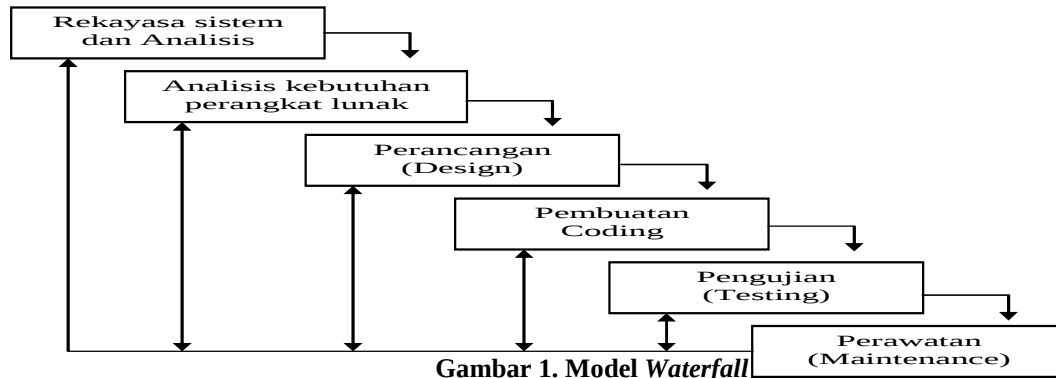
Gambar 1. Model Waterfall
