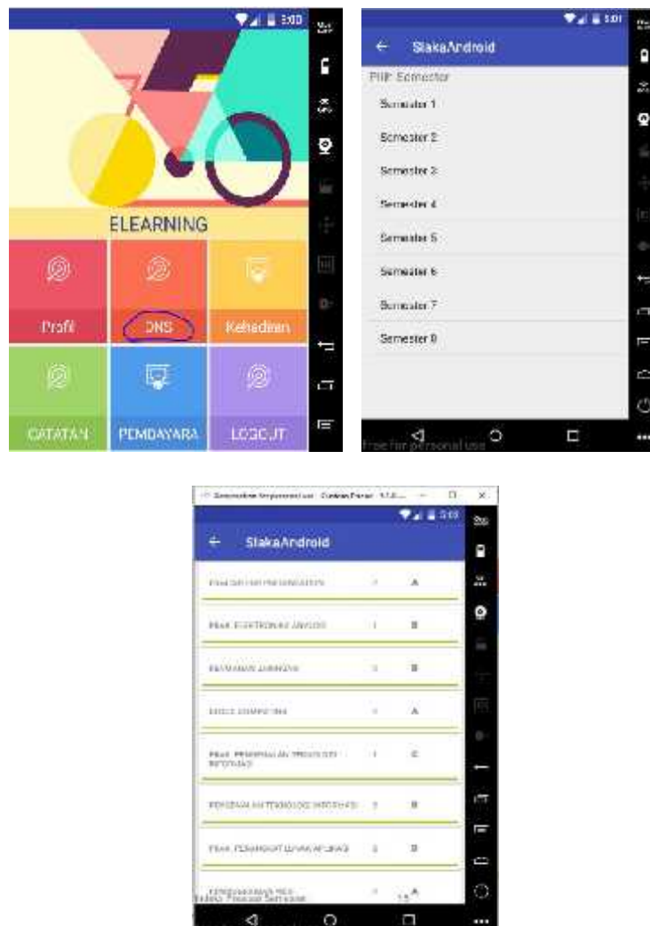
Gambar 5. DNS
