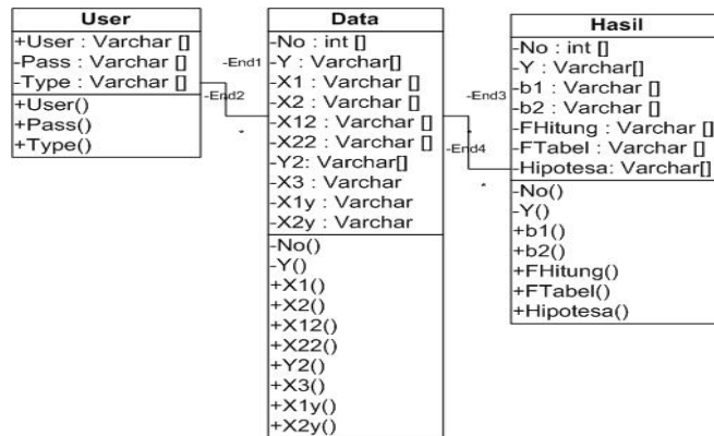
Gambar 3.3 Class Diagram
