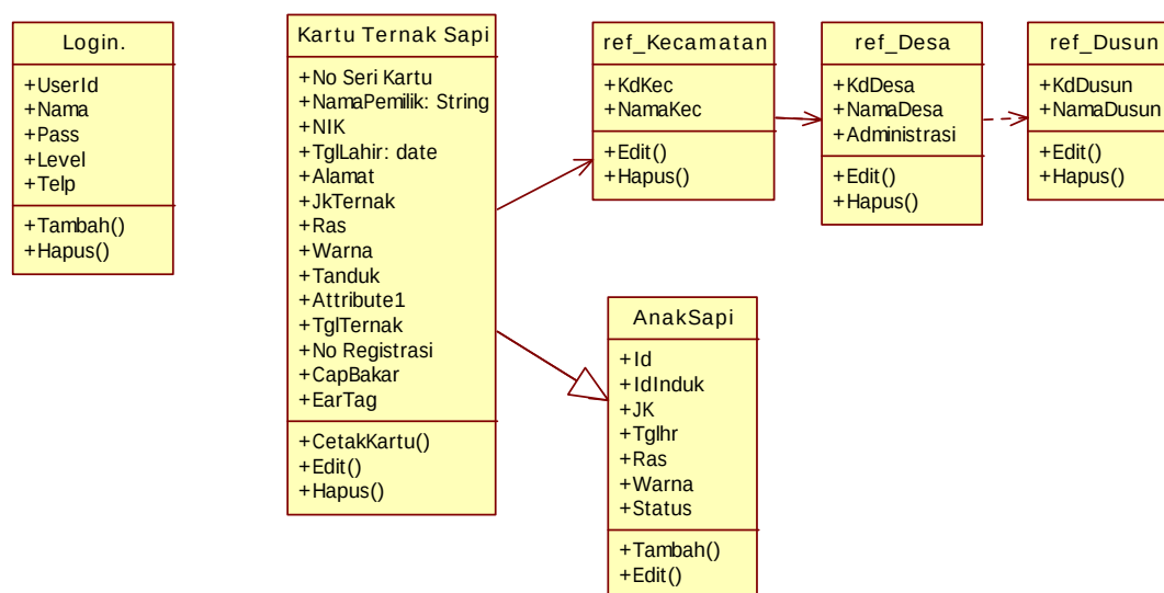
Gambar 4. Class Diagram
