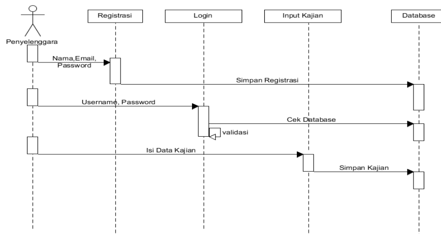
Gambar 3.4 Sequence Diagram User
