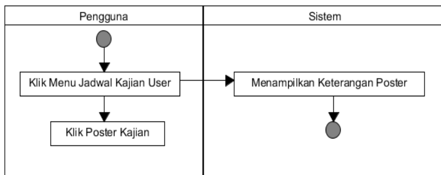
Gambar 3.7 Activity Diagram Jadwal Kajian User
