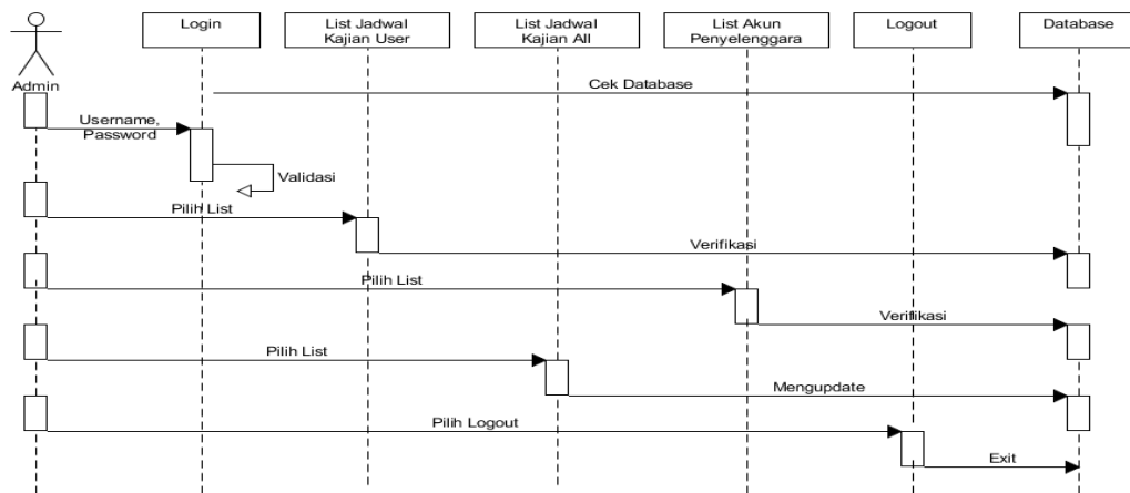
Gambar 3.3 Sequence diagram admin
