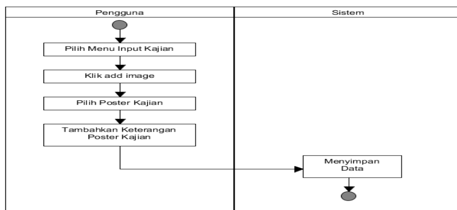
Gambar 3.8 Activity Diagram Input Kajian User
