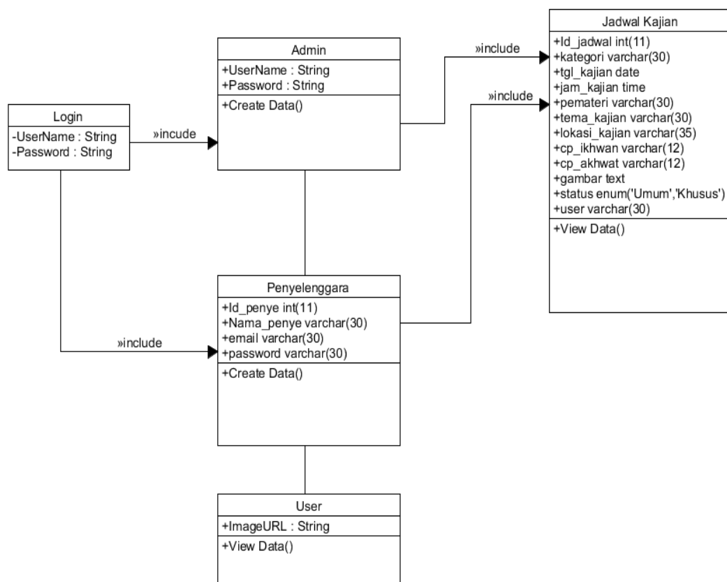
Gambar 3.2 Class Diagram Sistem Monitoring
