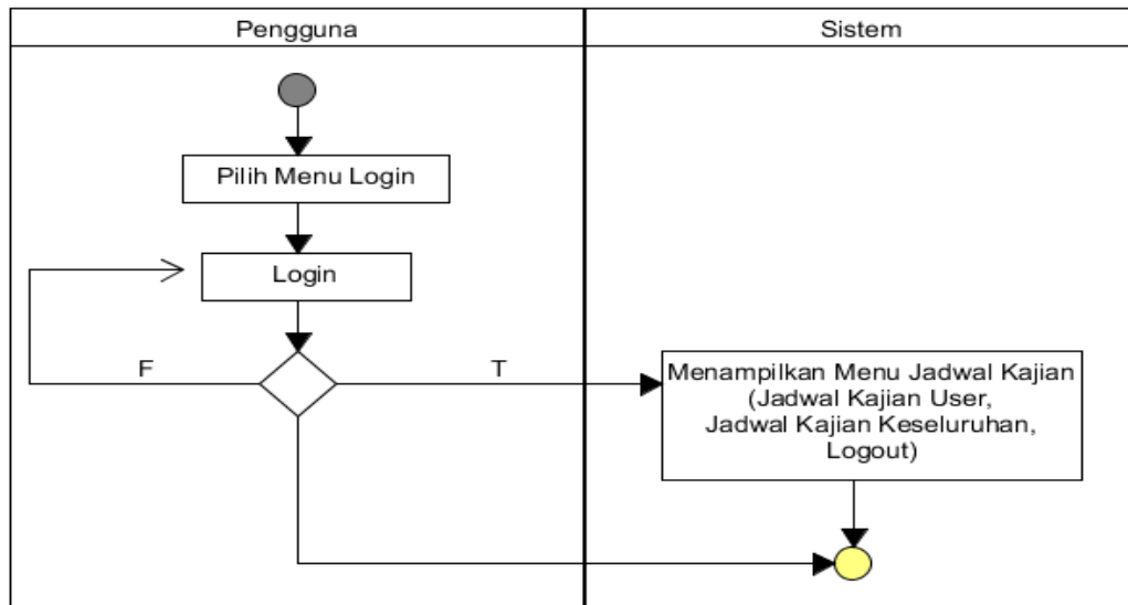
Gambar 3.6 Activity Diagram Login Admin
