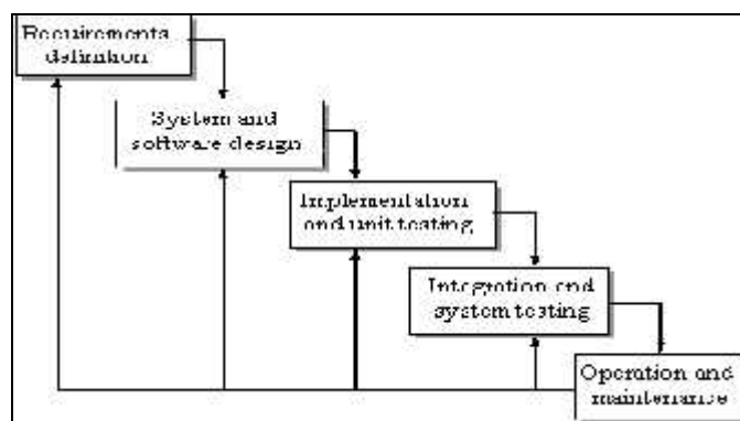
Gambar 1. Model waterfall
