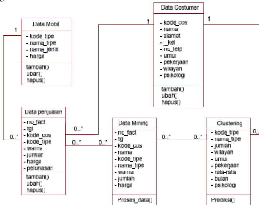
Gambar 4. Class diagram sistem
