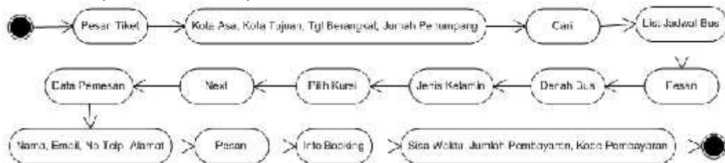
Gambar 4 Activity Diagram Pesan Tiket
