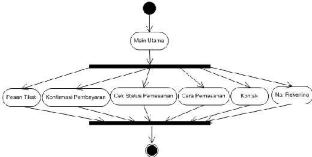
Gambar 3 Activity Diagram Menu Utama
