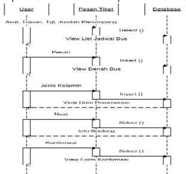
Gambar 6 Sequence Diagram Pesan Tiket
