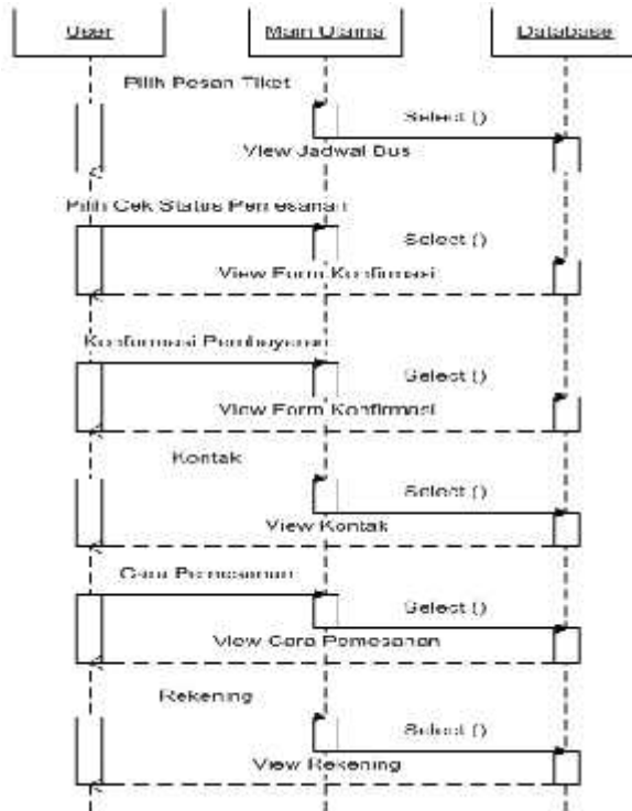
Gambar 5. Sequence Diagram Menu Utama
