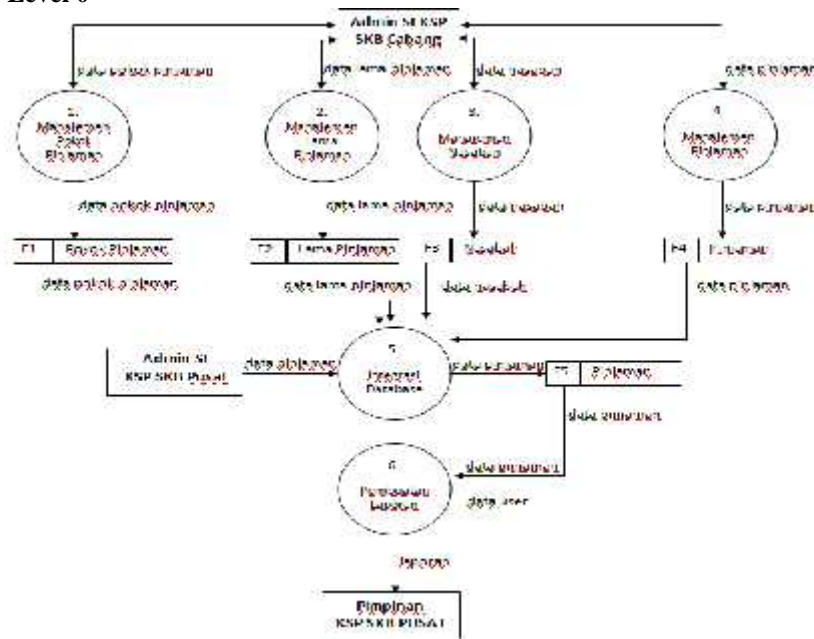
Gambar 3. Diagram level 0
