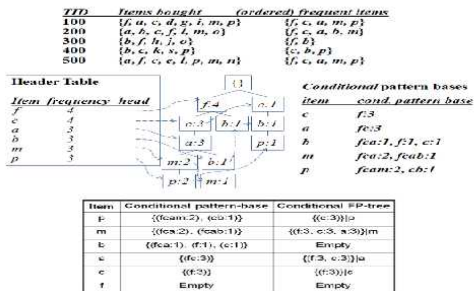
Gambar 3. Contoh Alur Algoritma FP-Growth
