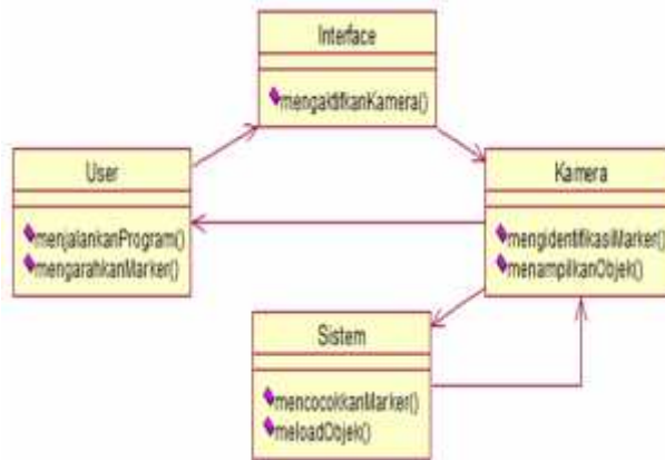
Gambar 7 Class Diagram
