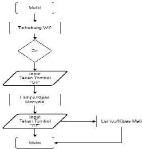
Gambar 5 Flowchar Prototype
