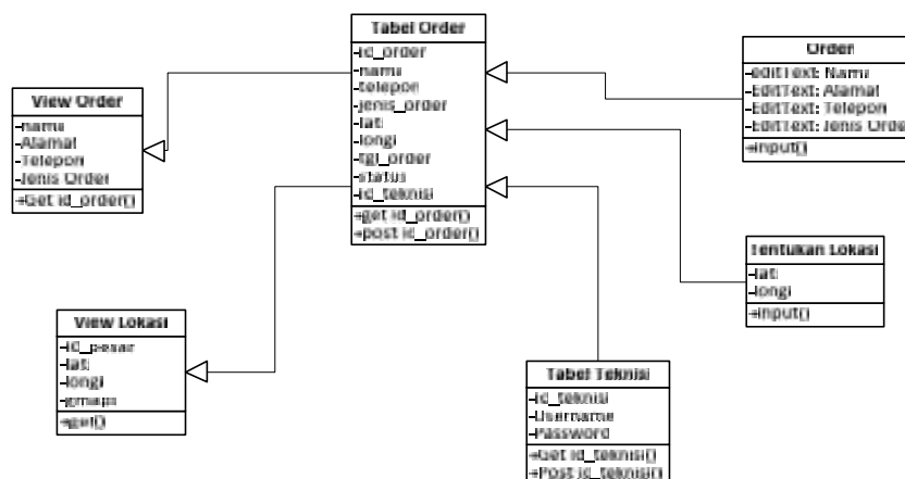
Gambar 3 : Class Diagram
