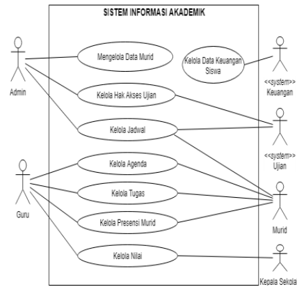
Gambar 3.1 Use Case Diagram Akademik
