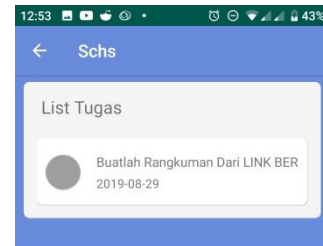
Gambar 4.50 Halaman Tugas
