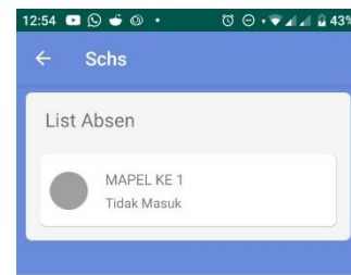
Gambar 4.49 Halaman Absen
