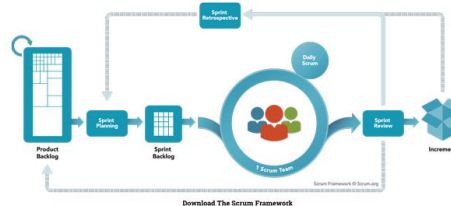
Gambar 2.1 Metode Scrum
