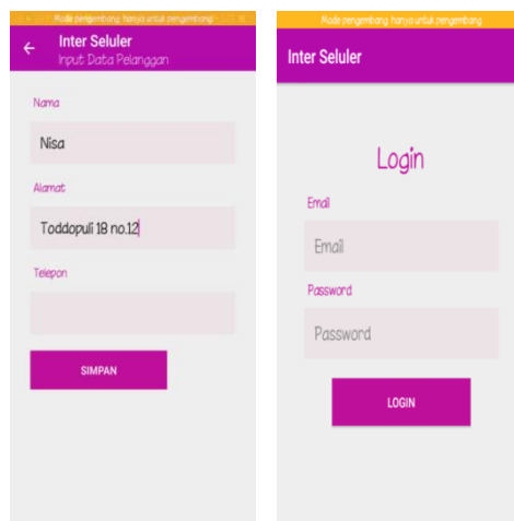
Gambar 10. Login User
