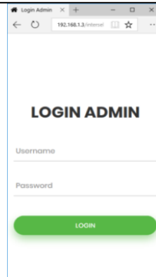
Gambar 5. Login Admin
