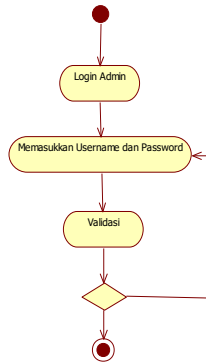
Gambar 3. Activity Diagram Login Admin
