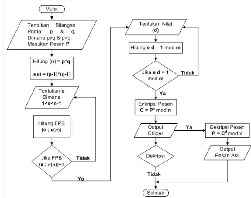
Gambar 3. Flowchart Proses Algoritma RSA
