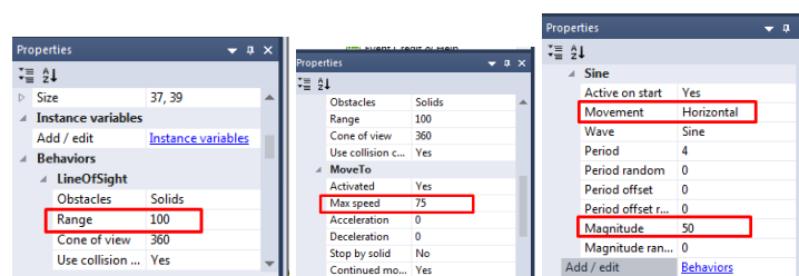
Gambar 7 Setting Behaviors Line Of Sight, MoveTo dan Sine Lebah
