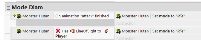
Gambar 15 Event Sheet Mode Diam
