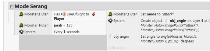
Gambar 13 Event Sheet Mode Serang
