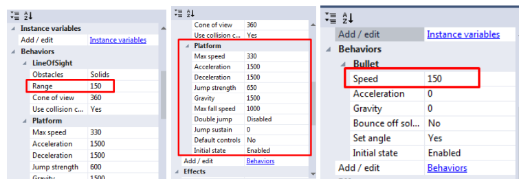
Gambar 9 Setting Behaviors Line Of Sight, Platform dan Peluru Katak
