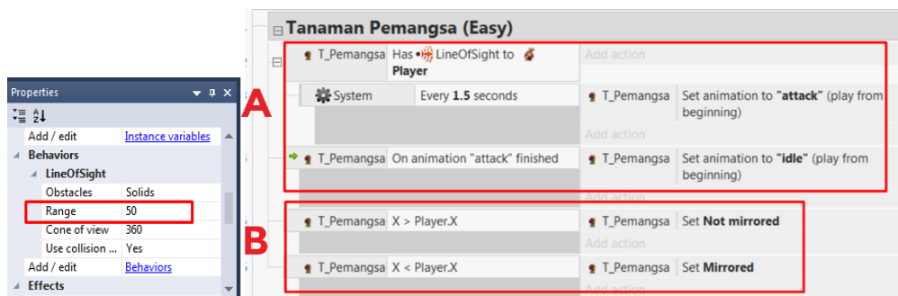
Gambar 6. Setting Behavior Tanaman dan Event Sheet Tanaman Pemangsa
