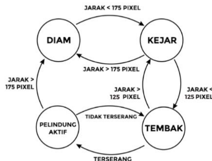
Gambar 5. Diagram Serangan Monster Hutan
