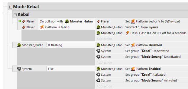
Gambar 14 Event Sheet Mode Kebal
