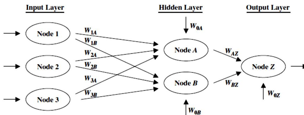
Gambar 2 : Model-ANN (Neural-net)
