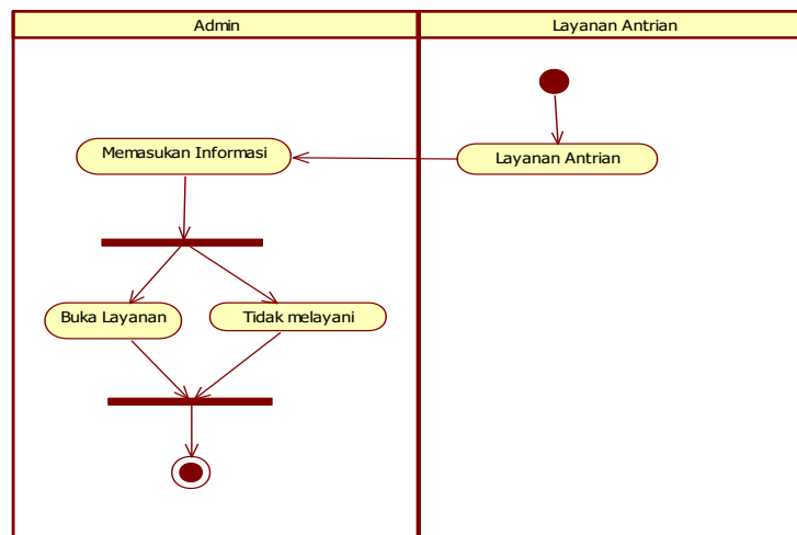
Gambar 3. Activity Diagram Layanan Antrian
