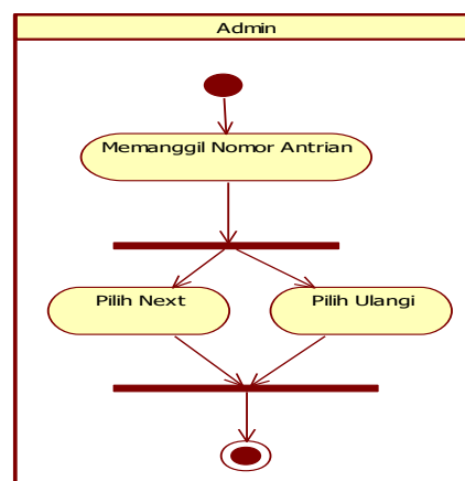
Gambar 4. Activity Diagram Memanggil Nomor Antrian
