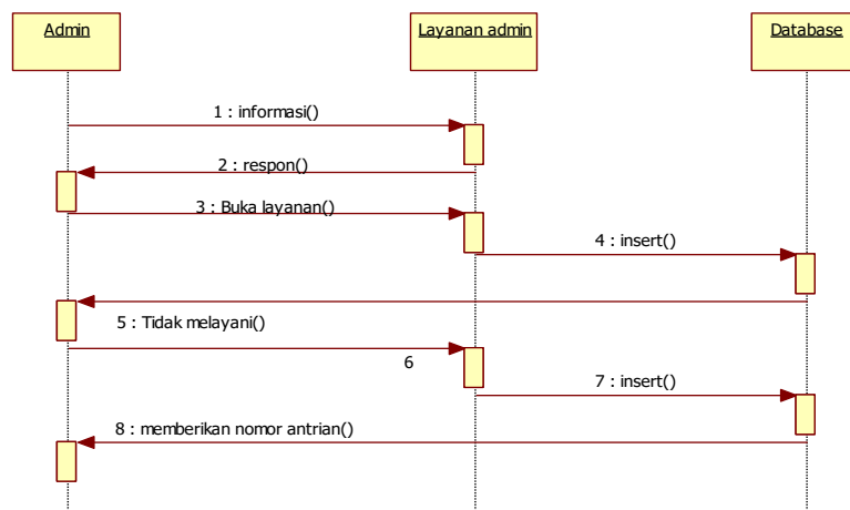
Gambar 2. Sequence Diagram Layanan Admin
