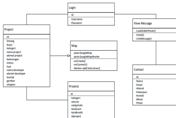
Gambar 3. Class Diagram
