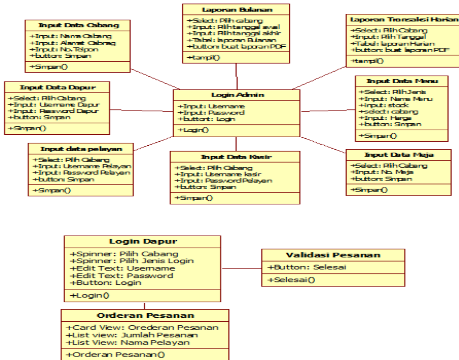
Gambar 3 Class Diagram
