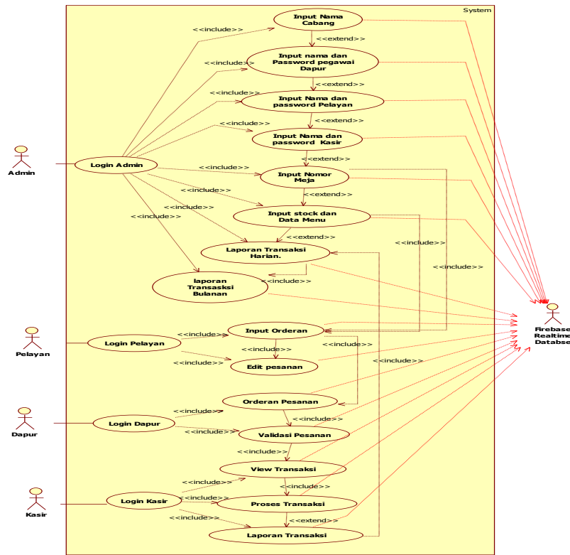
Gambar 2 Use Case Diagram Aplikasi E-Learning
