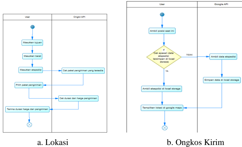
Gambar 2. Diagram Activity
