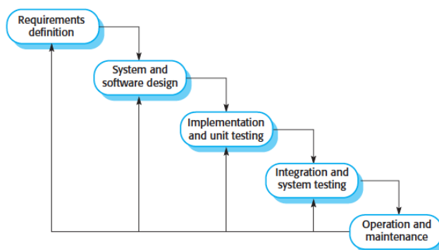
Gambar 1. Waterfall Model
