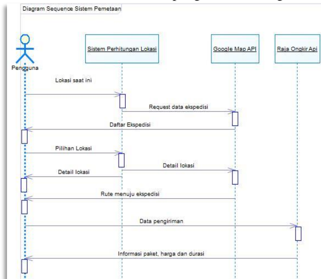
Gambar 3. Diagram Sequence
