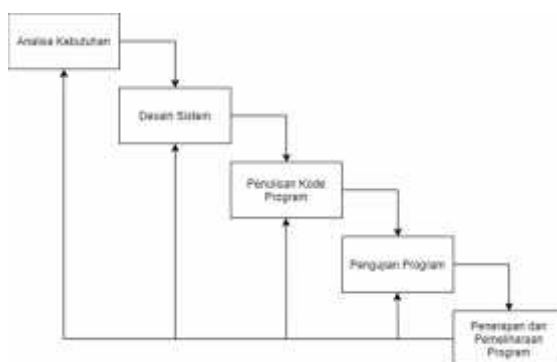
Gambar 1 Model Waterfall
