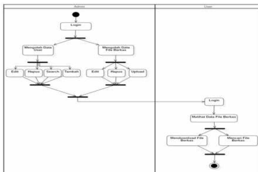
Gambar 2 Activity Diagram
