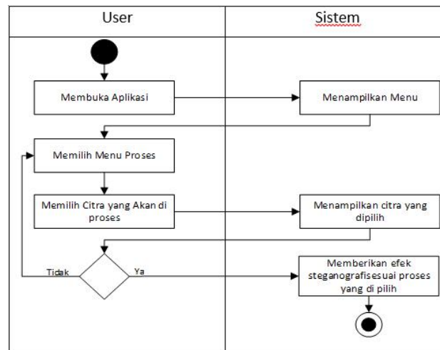
Gambar 3. Activity Diagram
