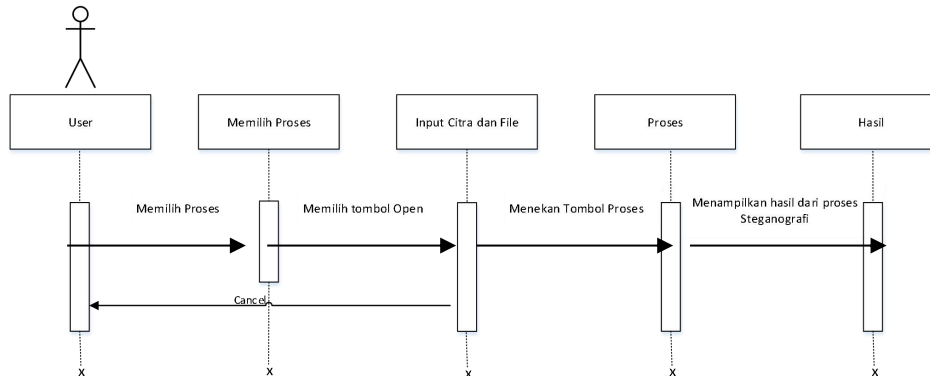
Gambar 4. Sequence Diagram
