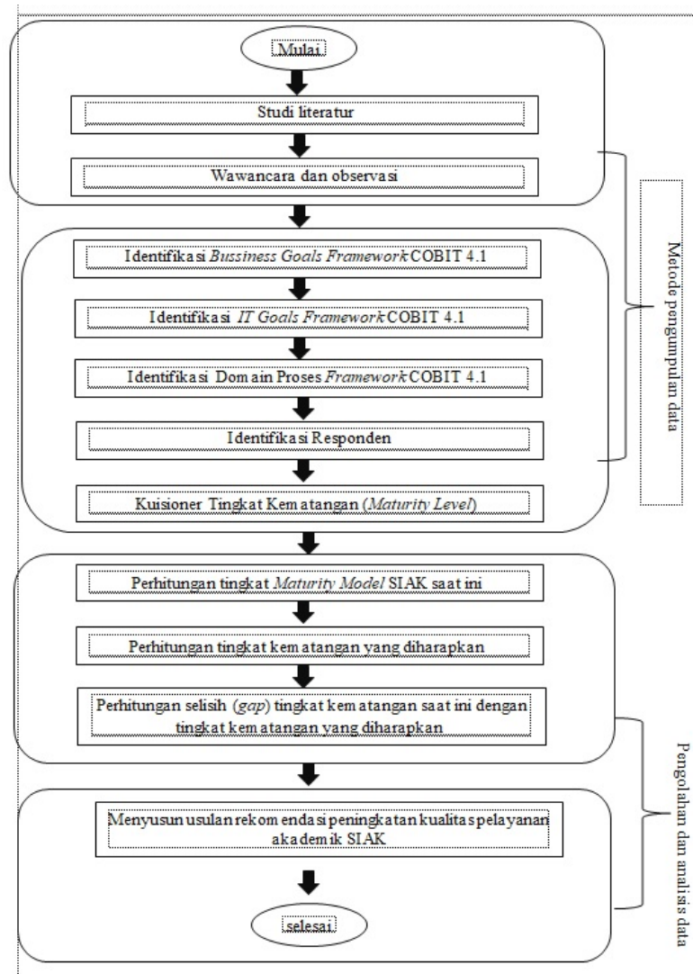
Gambar 2. Alur Penelitian
