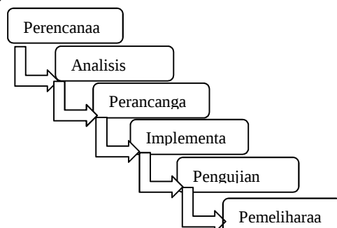
Gambar 1. Tahapan Waterfall [13]
