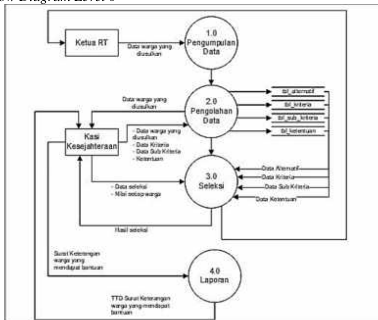
Gambar 4. DFD Level 0
