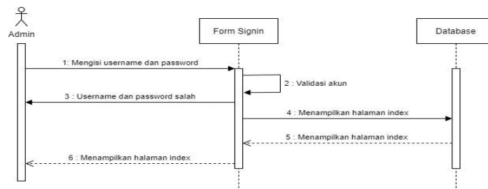
Gambar 6 Sequence Diagram Login Admin
