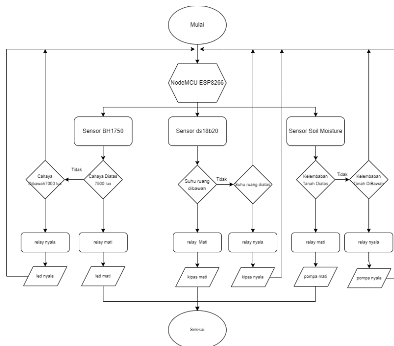
Gambar 1 Flowchart
