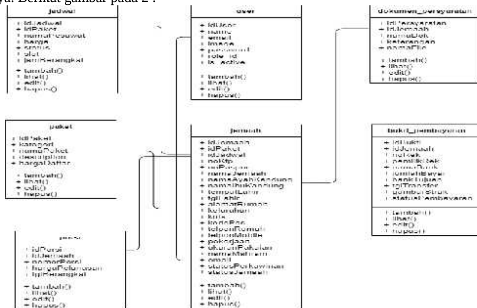
Gambar 2 Class Diagram
